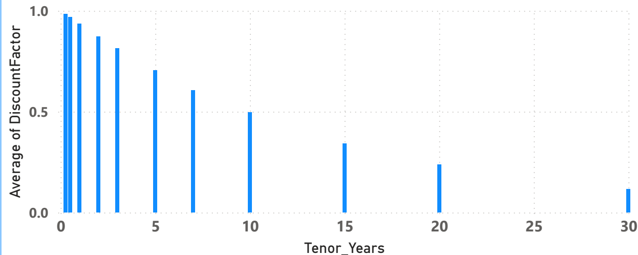
Discount Factor by Tenor
